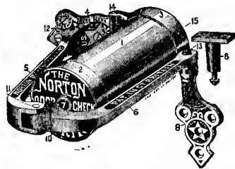
Fig. 2319. THE NORTON DOOR-CHECK.
